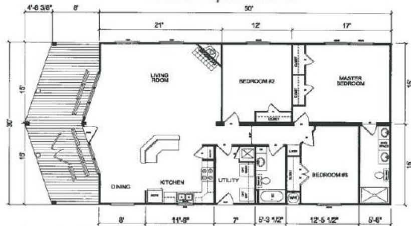
Spruce II - APH-906 - 1,529 Square feet plus covered deck as shown
